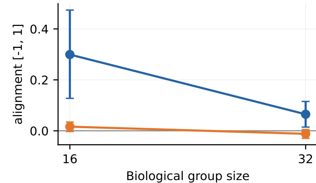
Prey | Escape alignment
