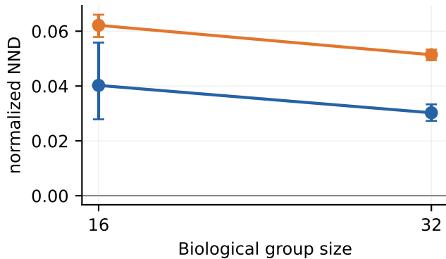
Collective | DoS (T-common)
