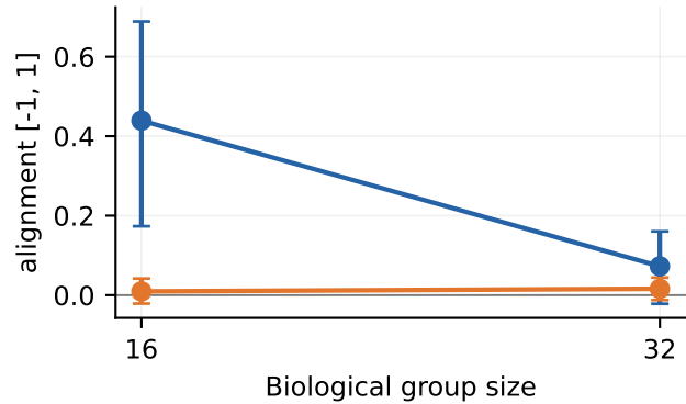
Predator | Pursuit alignment
