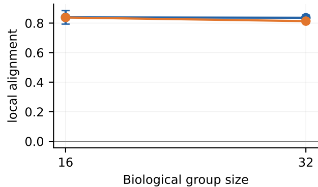
Collective | DoA (T-common)
