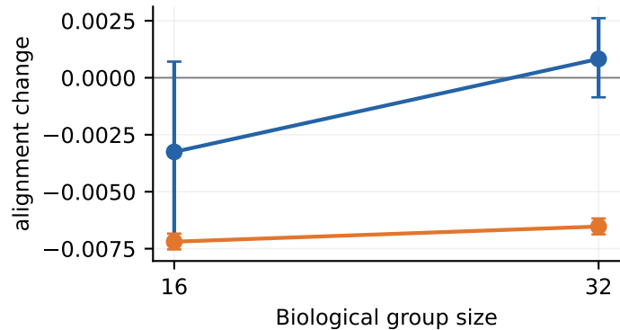
Prey | Prey reorientation R
